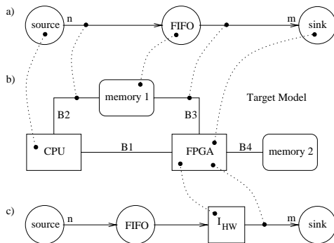
Figure 4. Logical channel refinement
