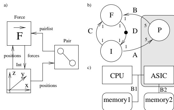
Figure 1. Dataflow graph for molecular dynamics simulation and target architecture
