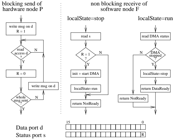
Figure 7. Interface refinement for channel B
