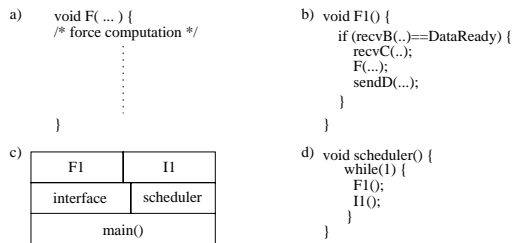
Figure 8. Implementation of the software partition of the molecular dynamics simulation application
