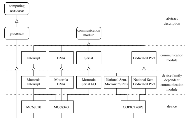
Figure 5. Object oriented modeling of processors
