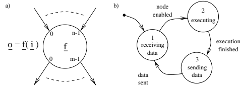
Figure 2. Abstract node model
