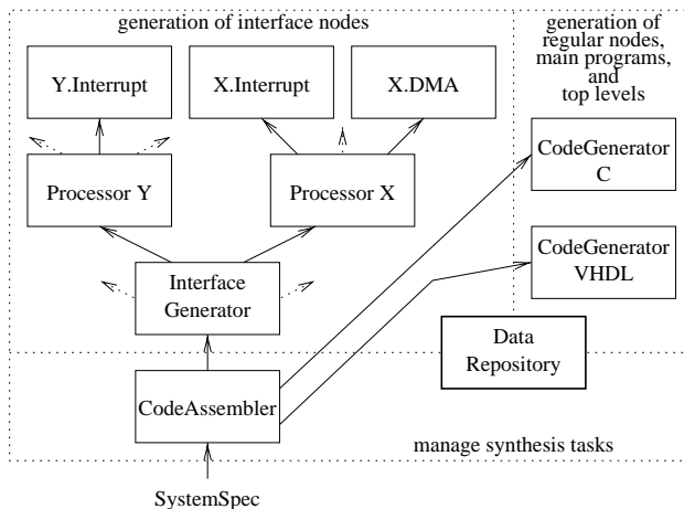
Figure 6. Detailed code generation
